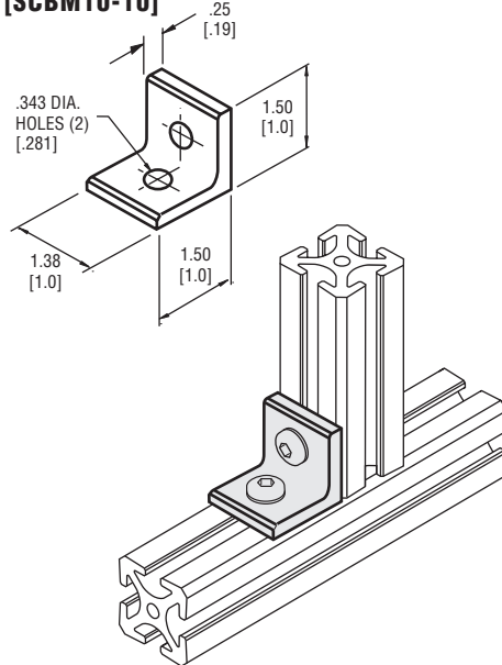
SCB15-15 [SCBM10-10]
