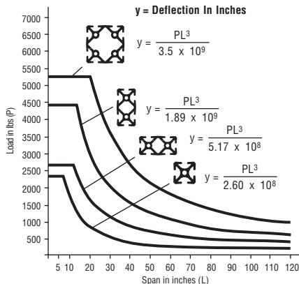
Fixed at one end, sliding at one end, load at center
