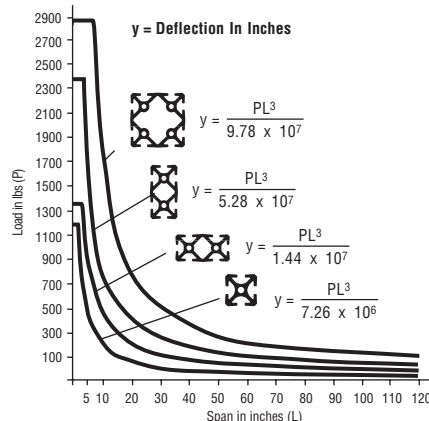
Fixed at one end, load at unsupported end
